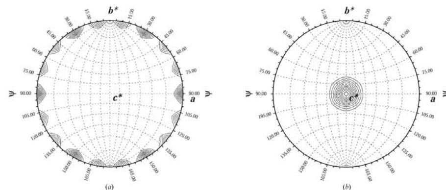
Figure 3 Stereographic projection of (a) the \kappa = 180 and (b) the \kappa = 40^\circ sections of the self-rotation function calculated using data in the range 10.0–2.4 Å and an integration radius of 20 Å. The peaks indicate a pseudo-ninefold non-crystallographic axis parallel to the crystallographic threefold screw axis.
